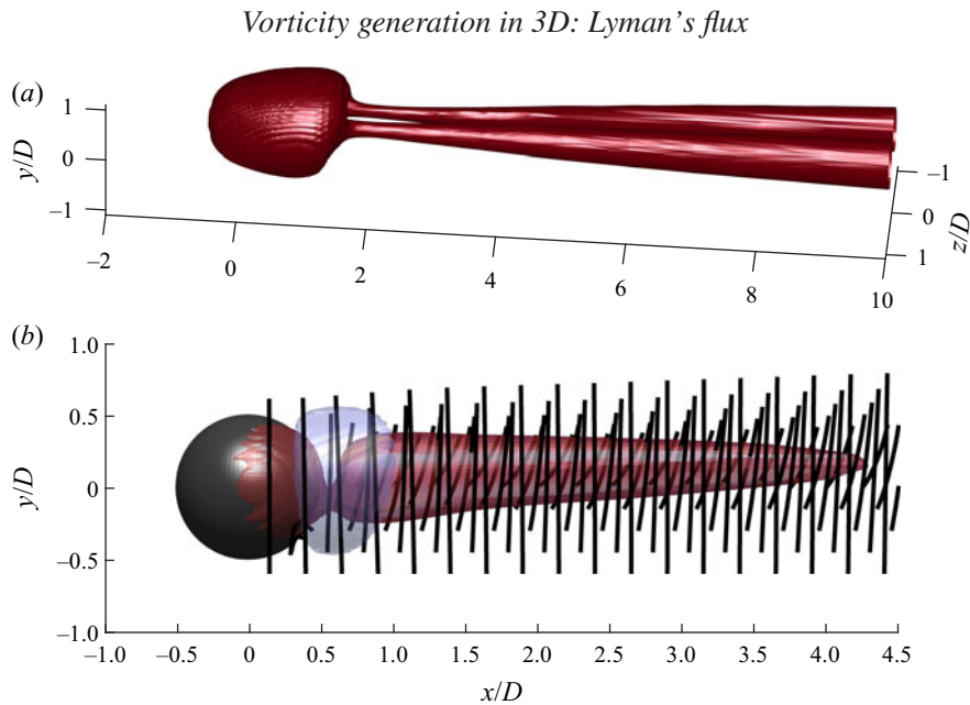
Figure 22. (a) Two streamwise-oriented vortices in the wake behind a sphere at Re = 250 , visualised using the \lambda_2 criterion. (b) Isosurfaces of streamwise vorticity: \omega_x/(U/D) = 0.3 (red), and \omega_x/(U/D) = -0.1 (blue), as well as representative vortex lines.
