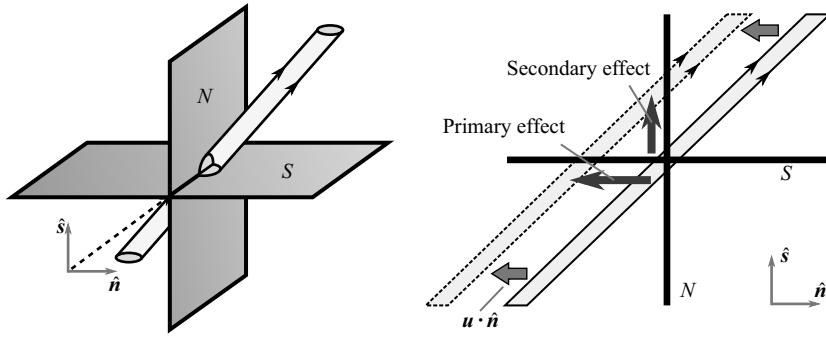
Figure 4. Transport of a vortex filament through two orthogonally intersecting surfaces. The term (\omega \cdot \hat{s})(u \cdot \hat{n}) occurs twice in the flux tensor, once representing the transport of (\omega \cdot \hat{s}) in the \hat{n} -direction (the primary effect), and a second time as the transport of (\omega \cdot \hat{n}) in the \hat{s} -direction (the secondary effect). Viscous terms in the Lyman–Huggins tensor are interpreted in an analogous manner.
