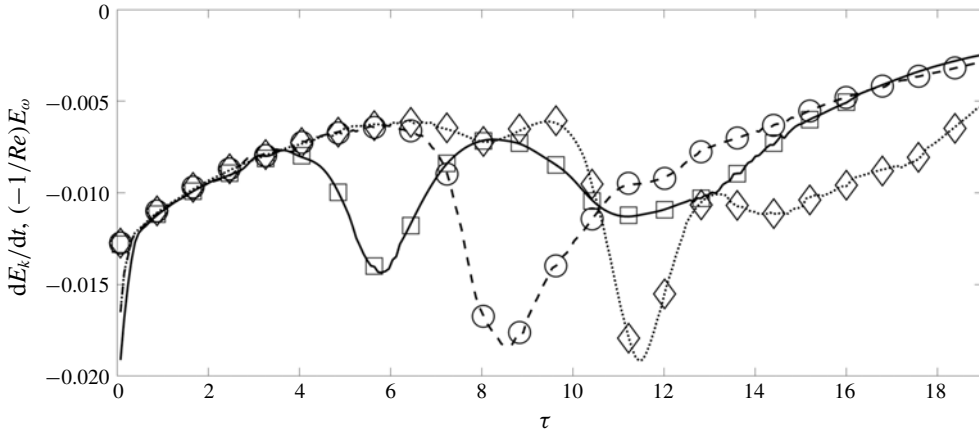
FIGURE 3. Validation study indicating that equation (2.7) is satisfied for all time steps of the solution for all three initial heights at Re = 2500 . The lines (—), (- - -) and ( \cdot\cdot\cdot ) correspond to the decay of global kinetic energy and the symbols ( \square ), ( \circ ) and ( \diamond ) correspond to the sign inverted global enstrophy scaled by the kinematic viscosity for h_0/b_0 = 5, 7.5 and 10 respectively. For visibility, the symbols are presented at intervals of \delta\tau = 5/\pi ; however, the largest error is no larger than 2.0% for all initial heights and \tau > 0.4 , once the initial velocity field evolves to satisfy the governing equations.
