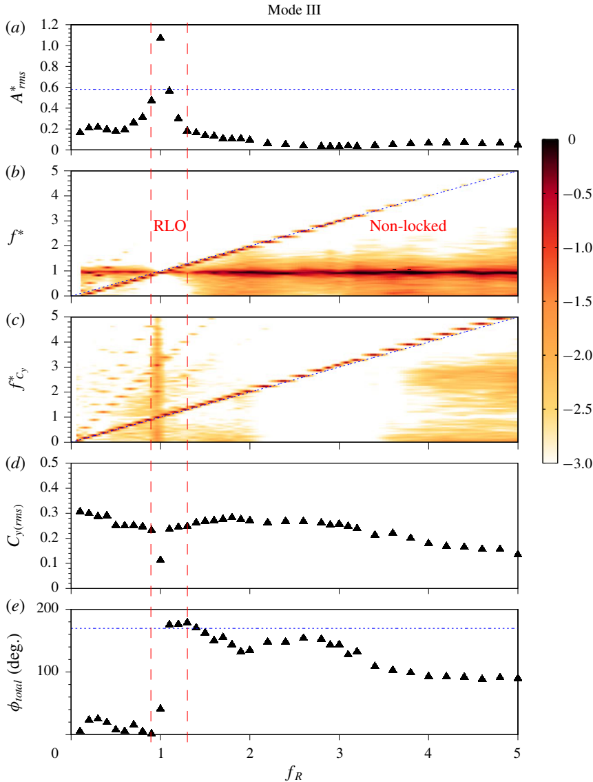
FIGURE 10. (Colour online) The response of an elastically mounted sphere with imposed rotary oscillations is presented as a function of forcing frequency ratio, f_R , at a fixed velocity ratio of \alpha_R = 1 in mode III ( U^* = 15 ). Refer to figure 4 for further details.
