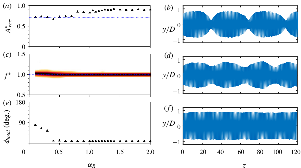
FIGURE 13. (Colour online) The response quantities of an elastically mounted sphere with the imposed rotary oscillations is presented as a function of velocity ratio, \alpha_R , at a fixed frequency ratio of f_R = 1 (a,c,e) for mode II. (b,d,f) The time traces of the sphere displacement for \alpha_R = 0.3 (b), \alpha_R = 0.6 (d) and \alpha_R = 1.2 (f).
