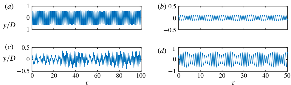
FIGURE 16. (Colour online) Time traces of the sphere displacement for f_R = 0.3 (a,c) and f_R = 0.9 (b,d) for a velocity ratio of \alpha_R = 1 . (a,c) Time traces for U^* = 8 and 15 , respectively. (b,d) Time traces for U^* = 6 and U^* = 10 , respectively.
